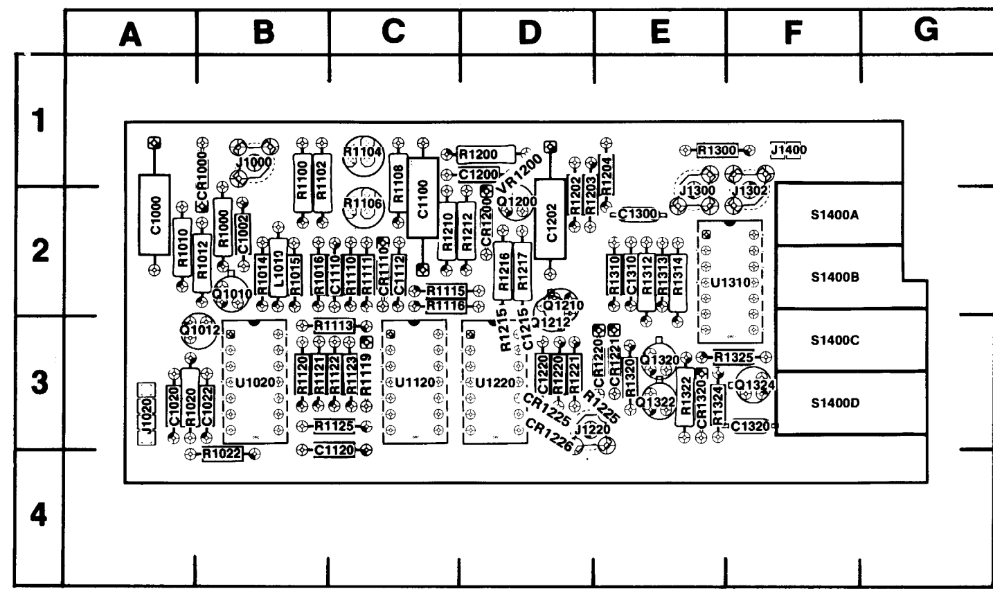
Fig. 8-5. Auxiliary Board (A12 Assy).
